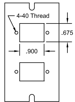
DP012 For (2) Modular L-COM Couplers
