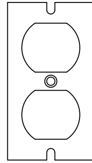
DP004 Device Plate For Duplex Receptacle
