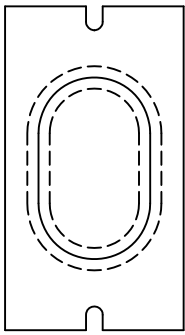
DP005 For 1" x 1 3/4" Grommet
