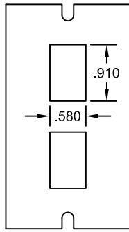
DP006 For (2) Modular Jack Couplers
