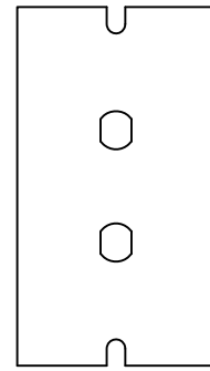
DP008 For (2) "ST" Style Connectors
