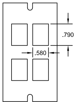
DP010 For (4) Tyco SL-110 Jacks
