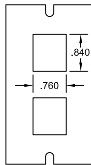
DP011 For (2) Modular Jack Couplers
