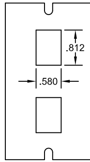
DP007 For (2) Modular Jack Couplers
