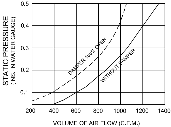
AIR FLOW CHARACTERISTICS
