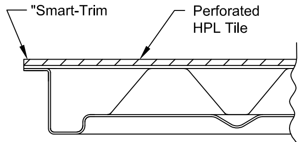
PARTIAL SECTION VIEW
