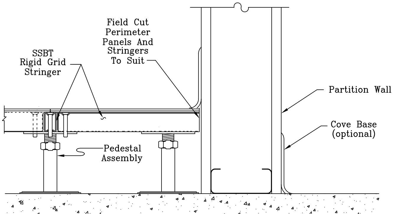
PARTITION THROUGH TO SUB-FLOOR
